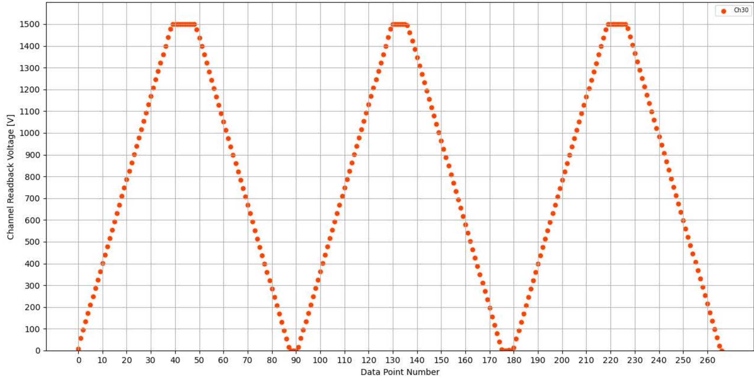
Voltage Ramp Test (Python) Bd #339, Slot #10, Ch #30
