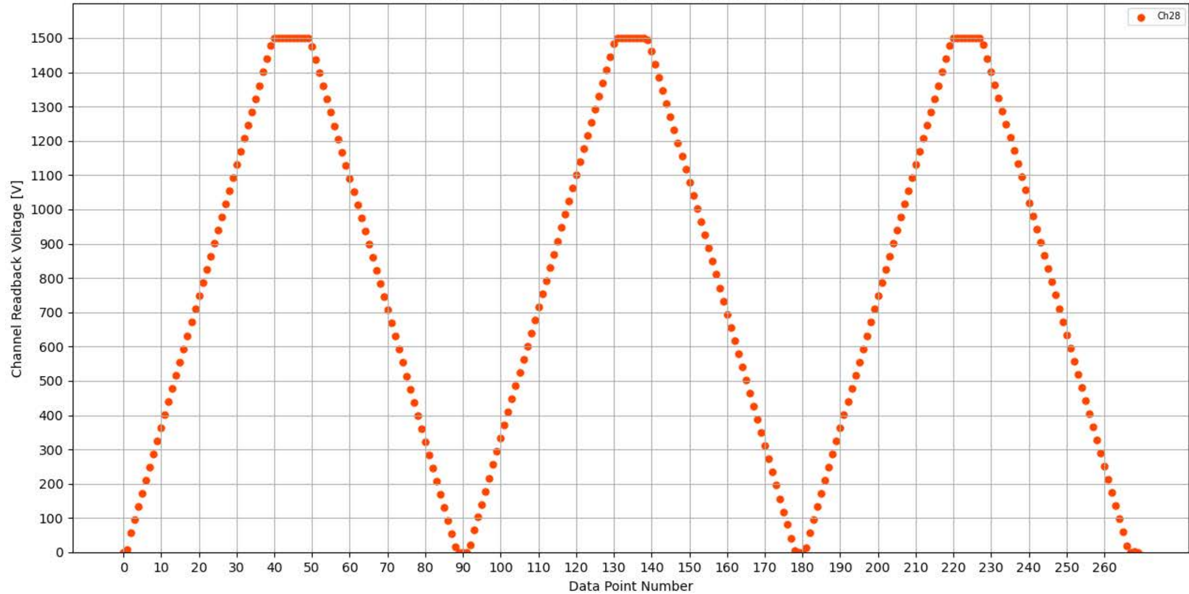
Voltage Ramp Test (Python) Bd #339, Slot #10, Ch #28
