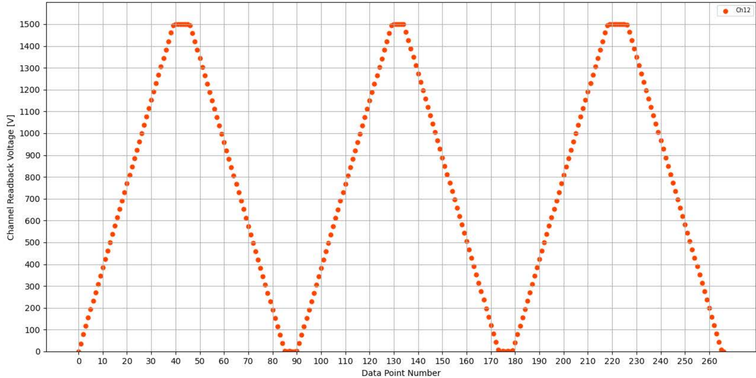
Voltage Ramp Test (Python) Bd #339, Slot #10, Ch #12
