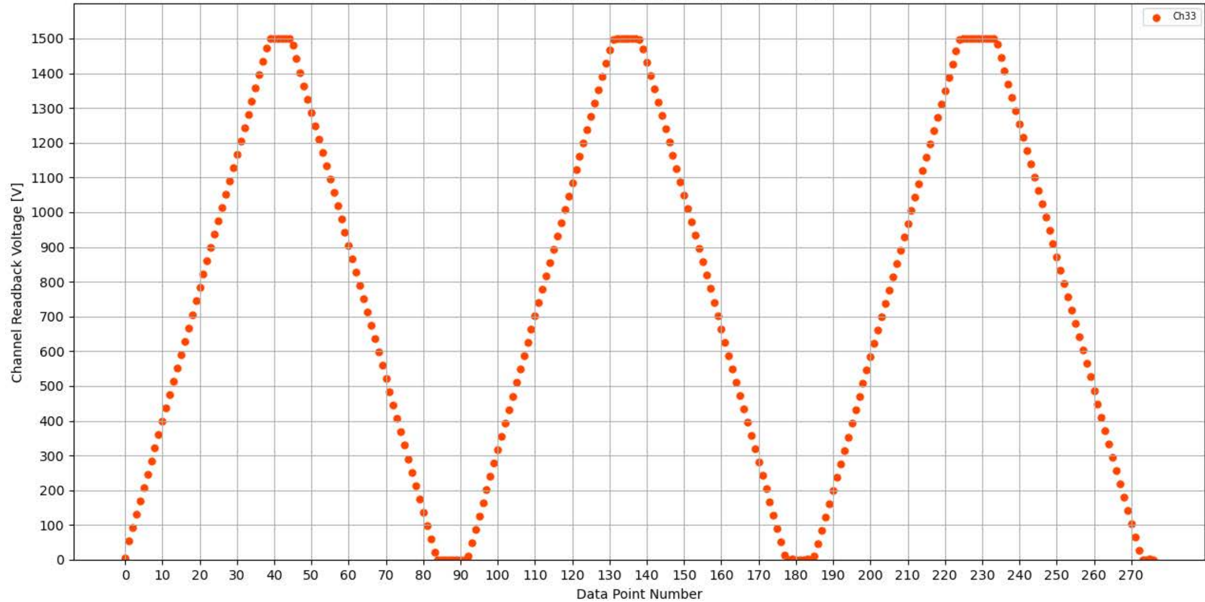
Voltage Ramp Test (Python) Bd #339, Slot #10, Ch #33
