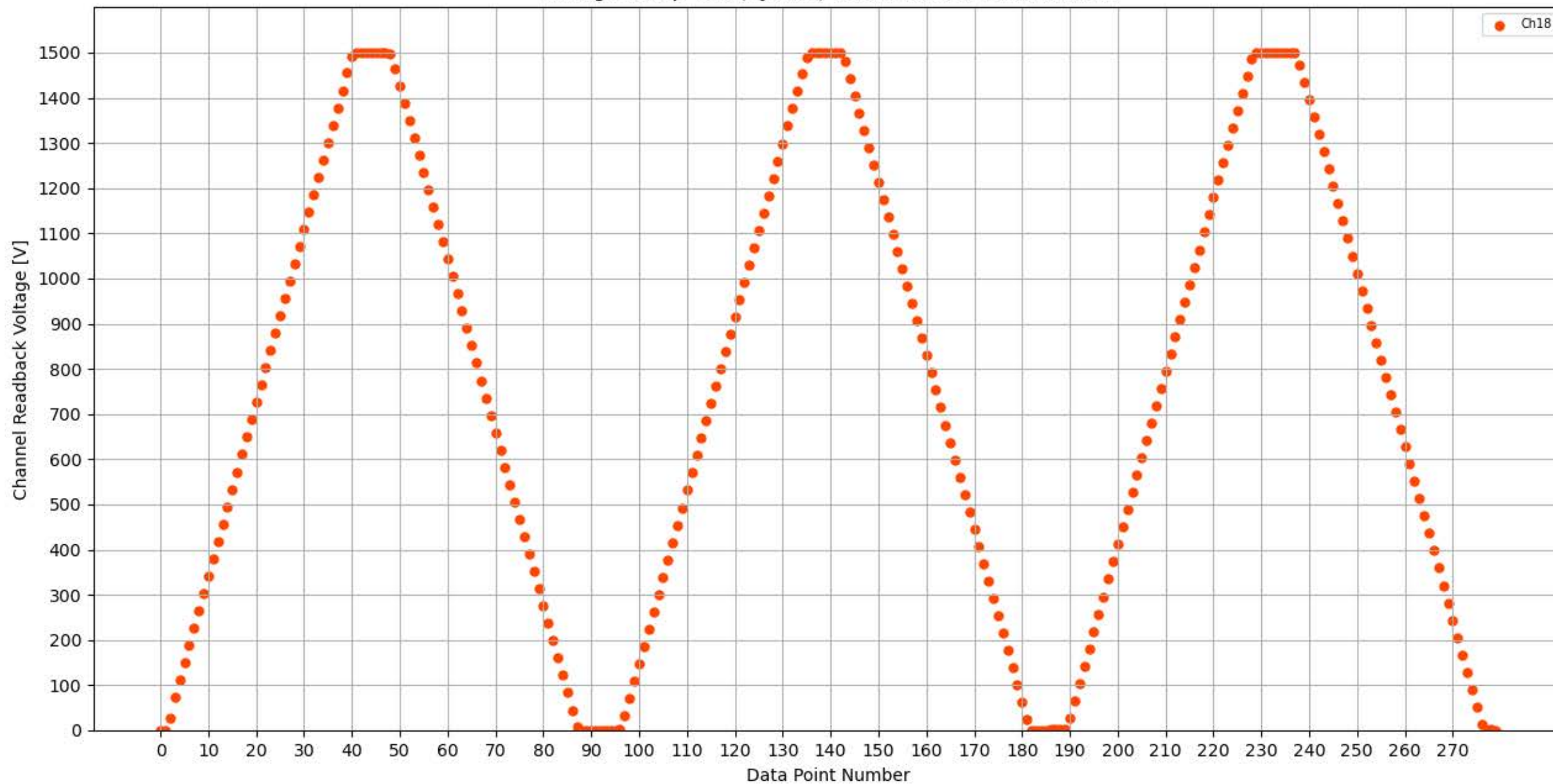
Voltage Ramp Test (Python) Bd #339, Slot #10, Ch #18
