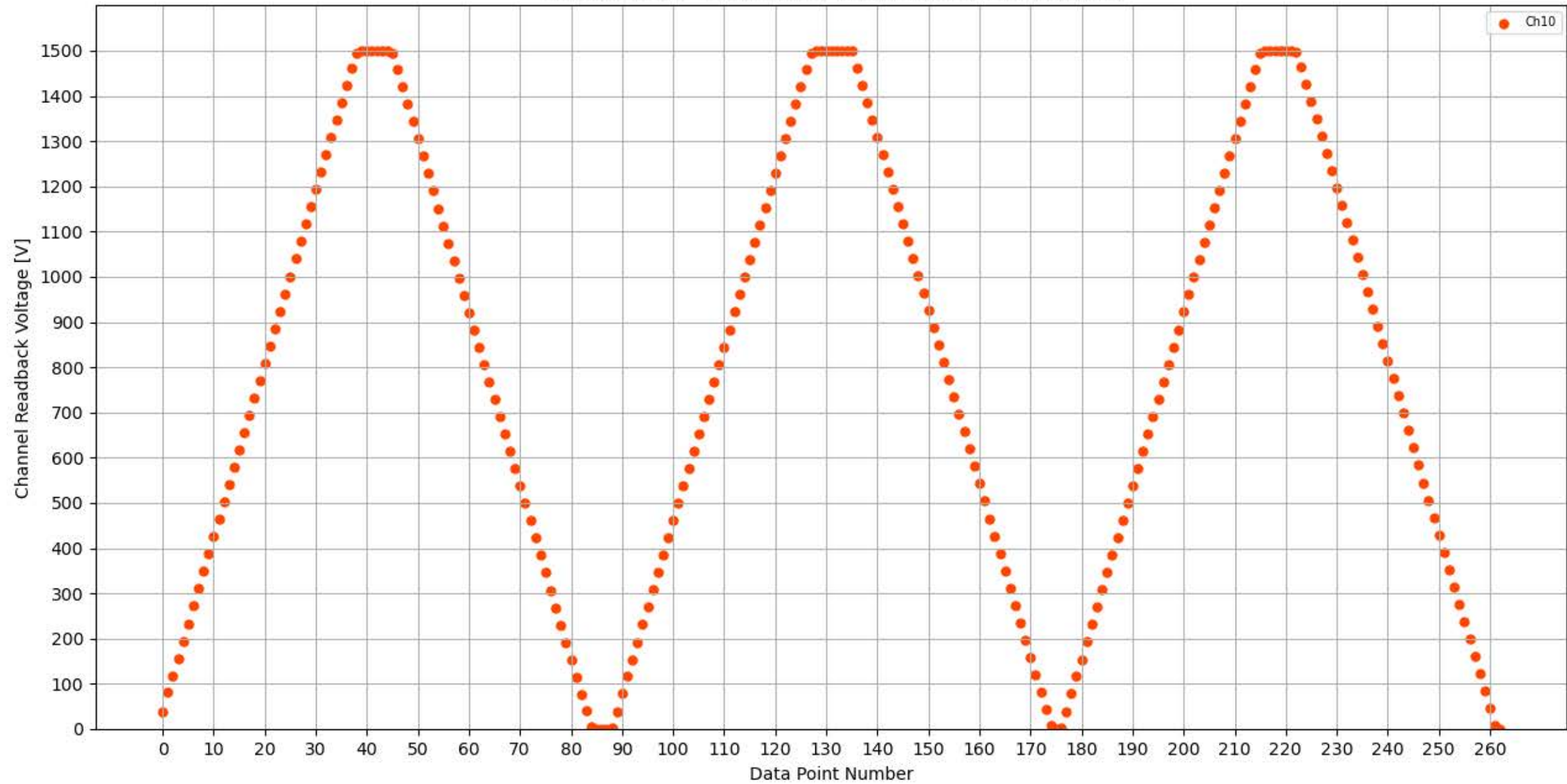
Voltage Ramp Test (Python) Bd #339, Slot #10, Ch #10
