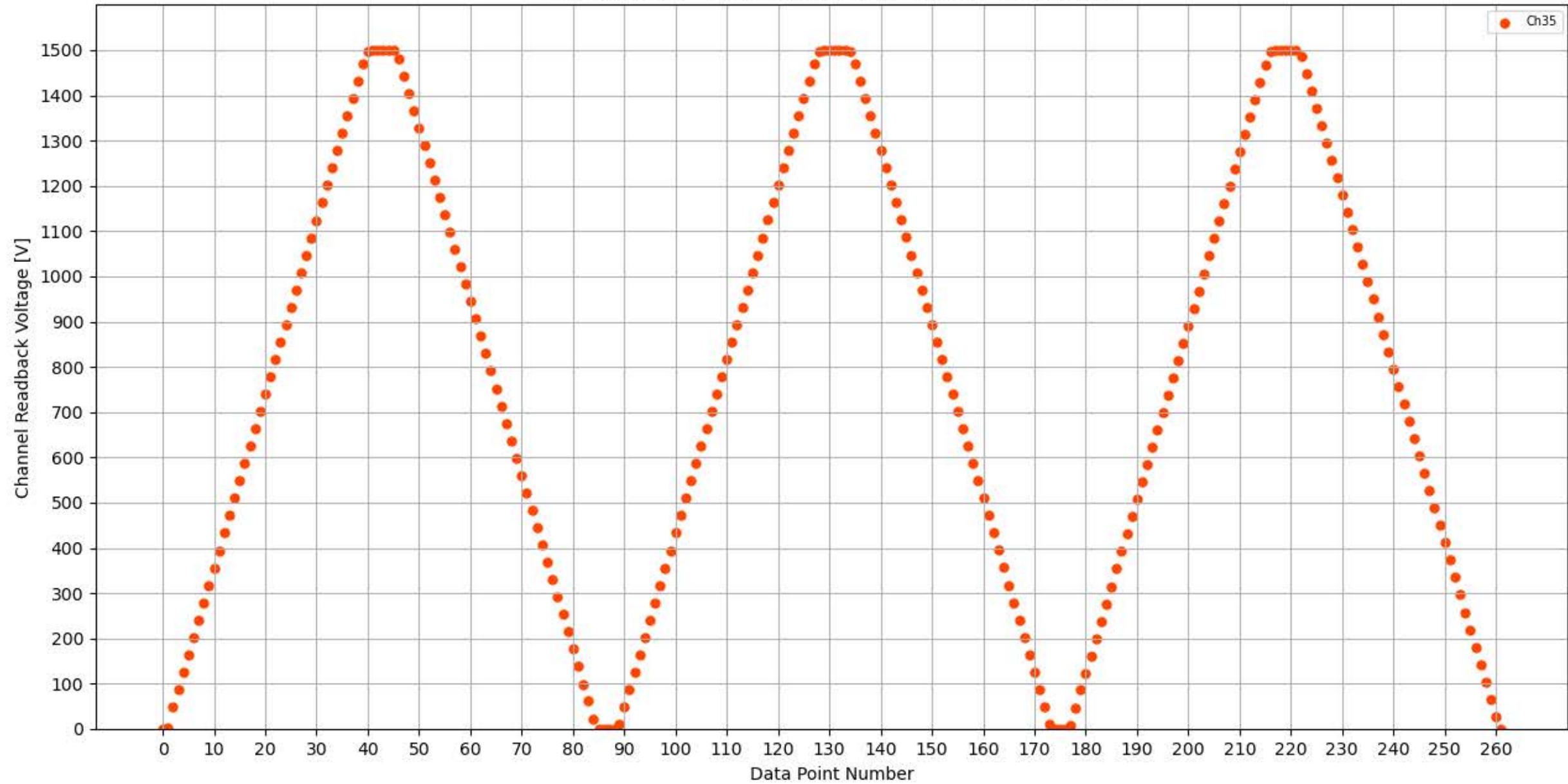
Voltage Ramp Test (Python) Bd #339, Slot #10, Ch #35
