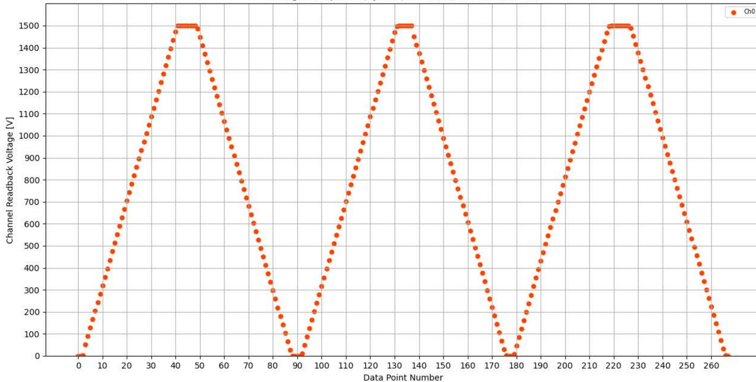
Voltage Ramp Test (Python) Bd #339, Slot #10, Ch #0
