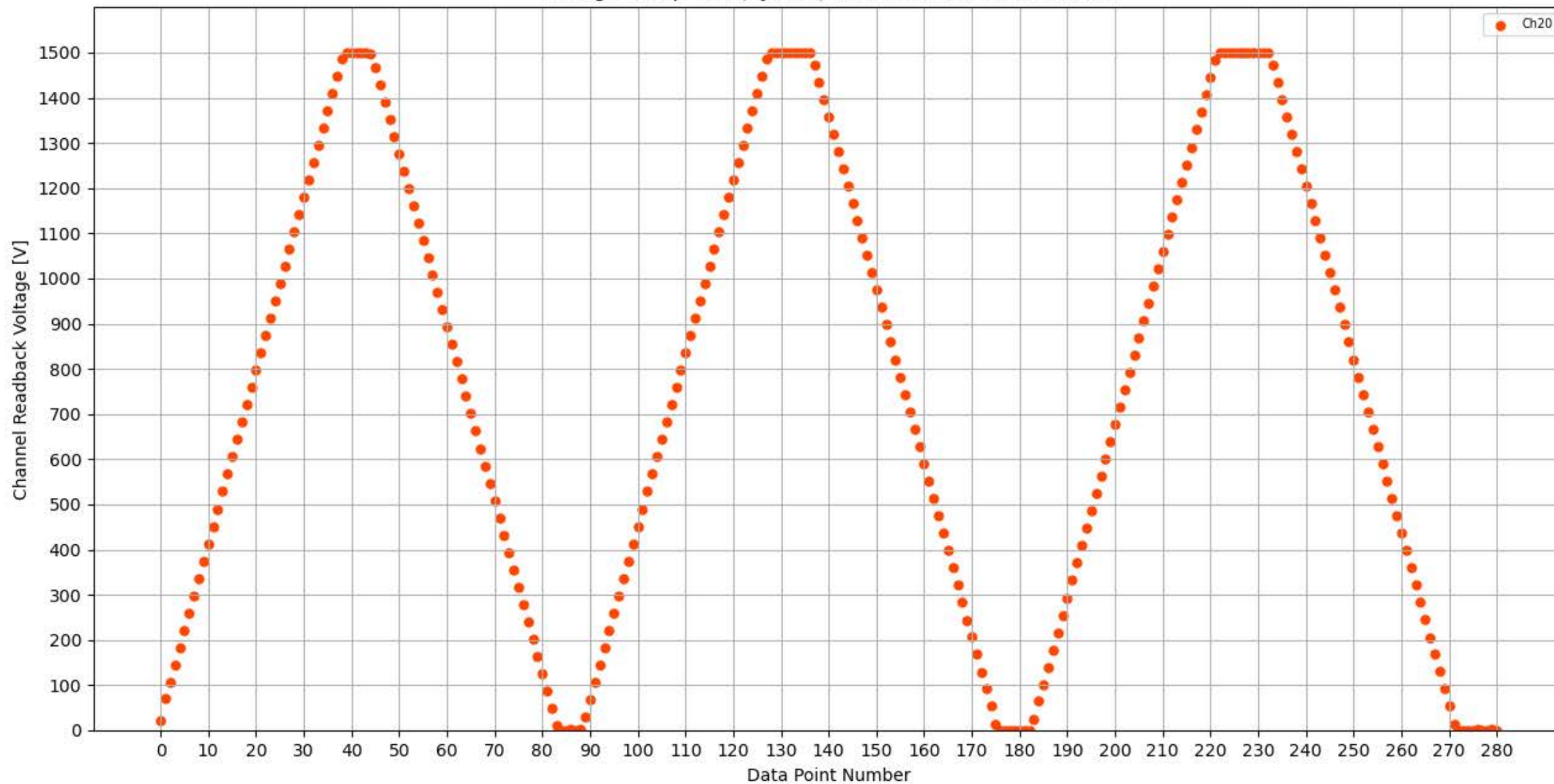
Voltage Ramp Test (Python) Bd #339, Slot #10, Ch #20
