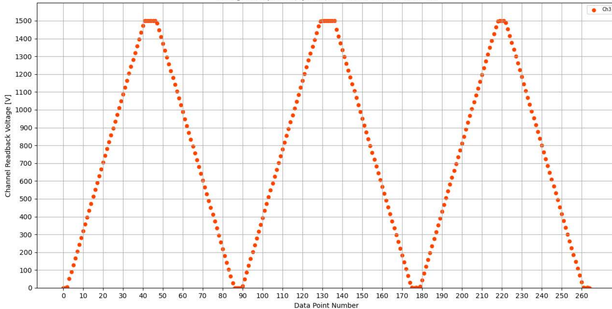
Voltage Ramp Test (Python) Bd #339, Slot #10, Ch #3
