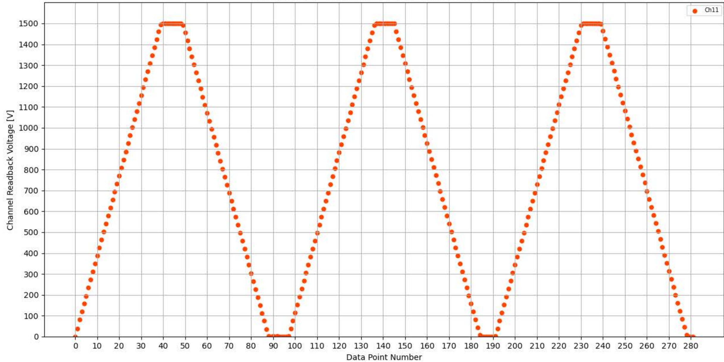
Voltage Ramp Test (Python) Bd #339, Slot #10, Ch #11
