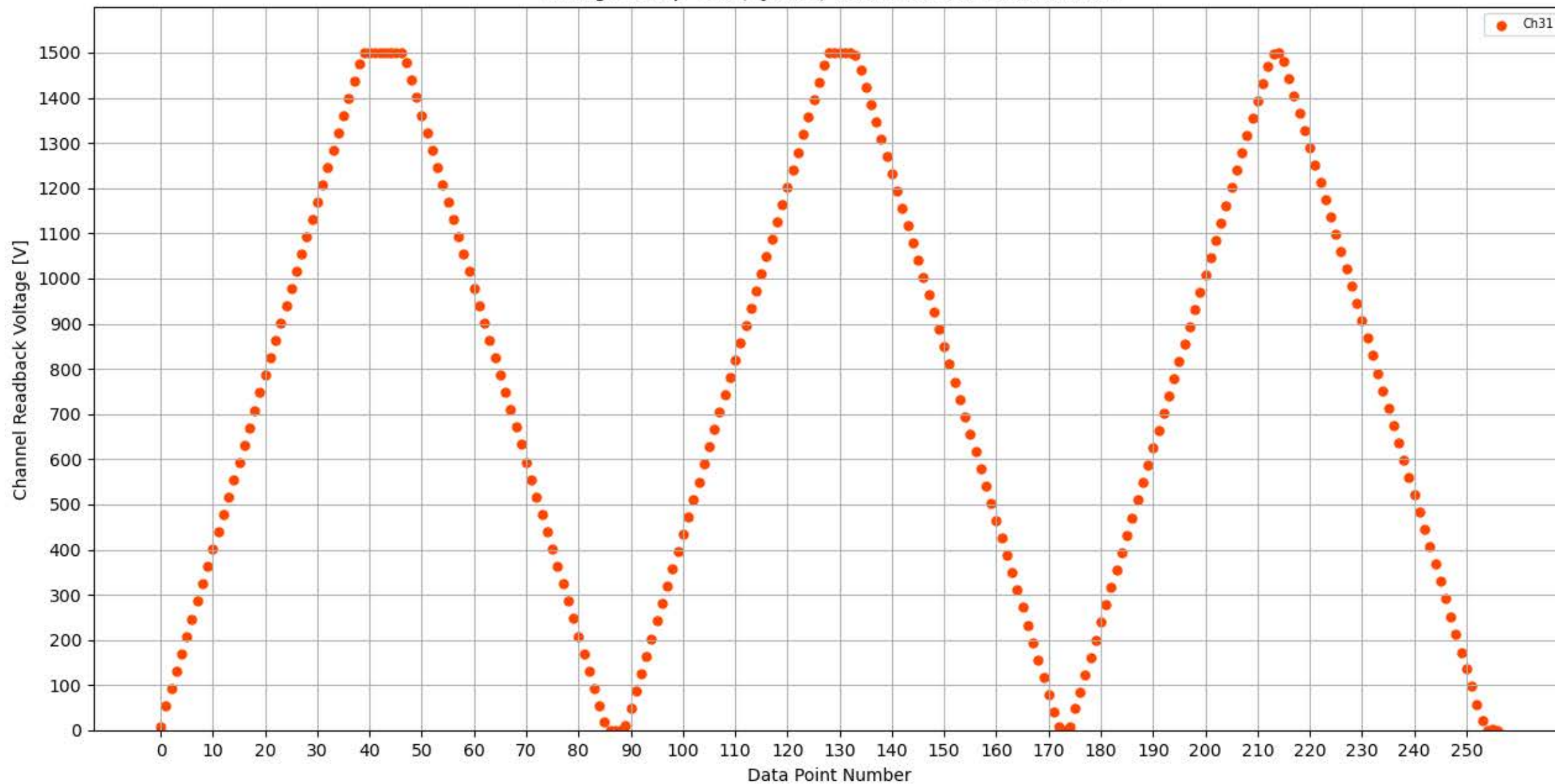
Voltage Ramp Test (Python) Bd #339, Slot #10, Ch #31
