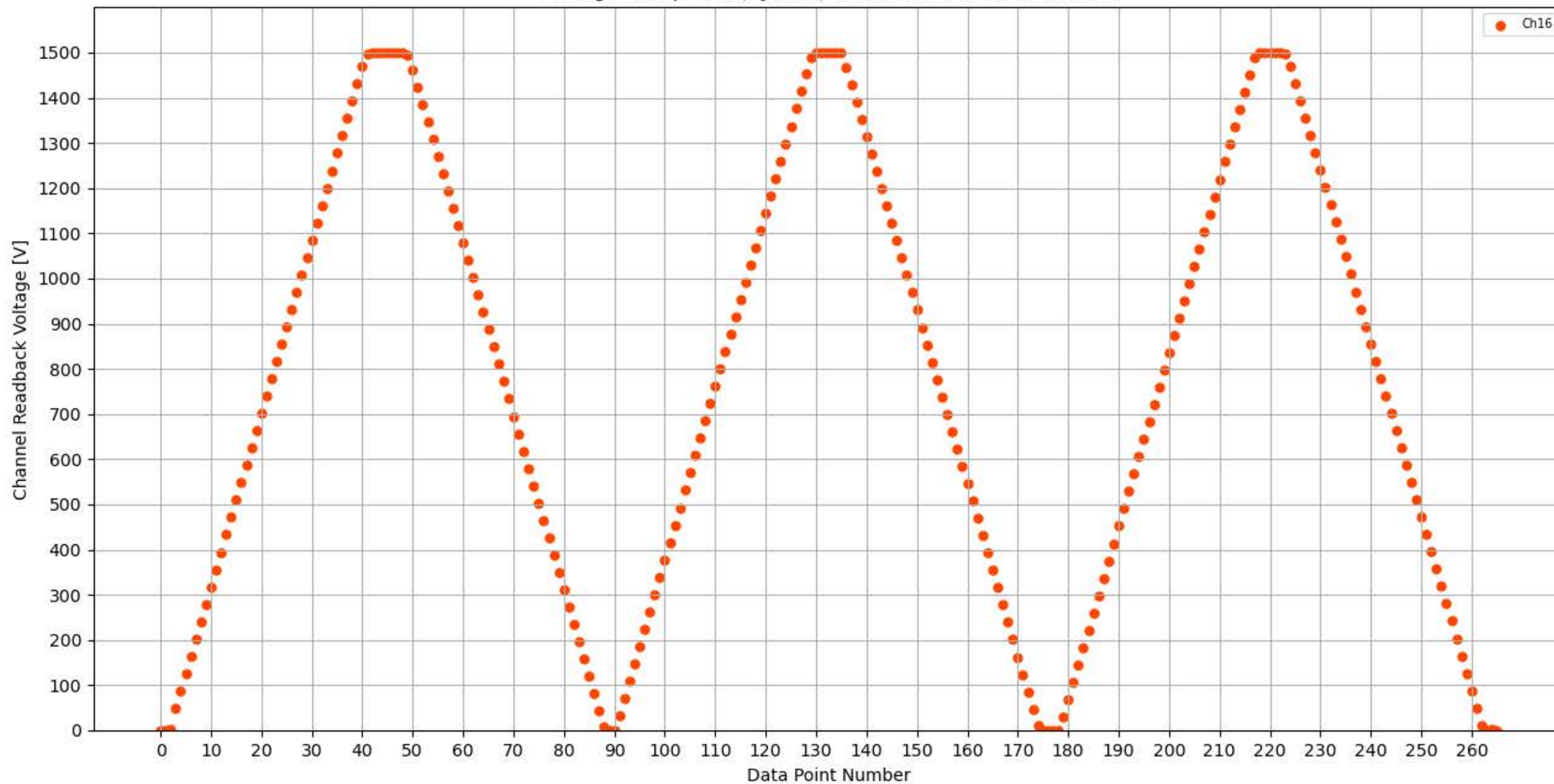
Voltage Ramp Test (Python) Bd #339, Slot #10, Ch #16
