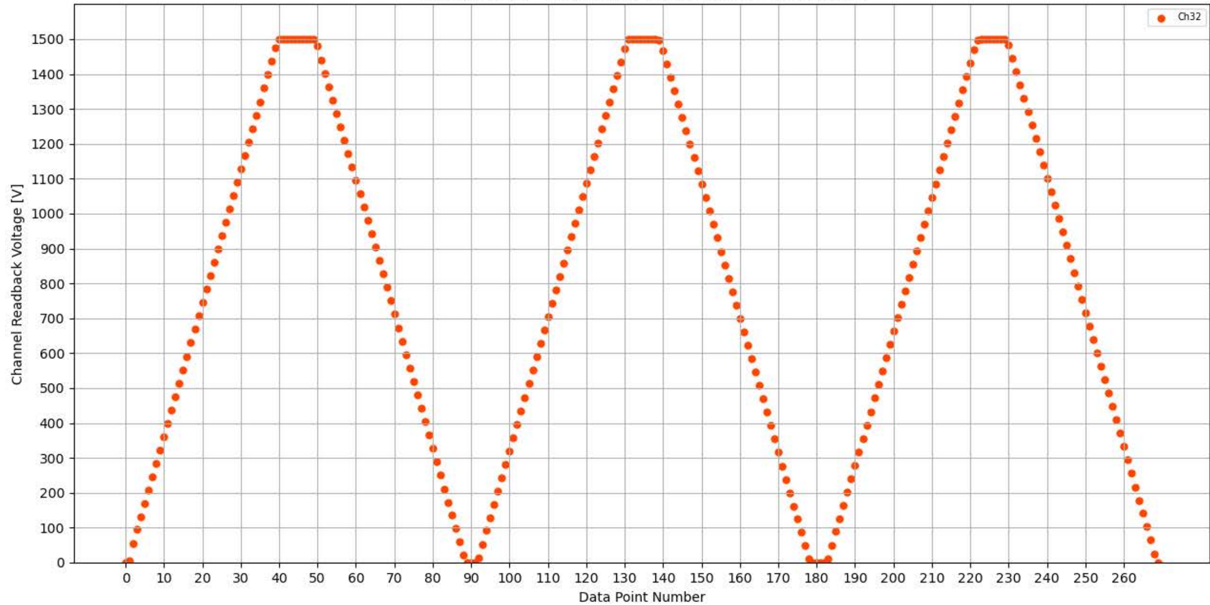
Voltage Ramp Test (Python) Bd #339, Slot #10, Ch #32
