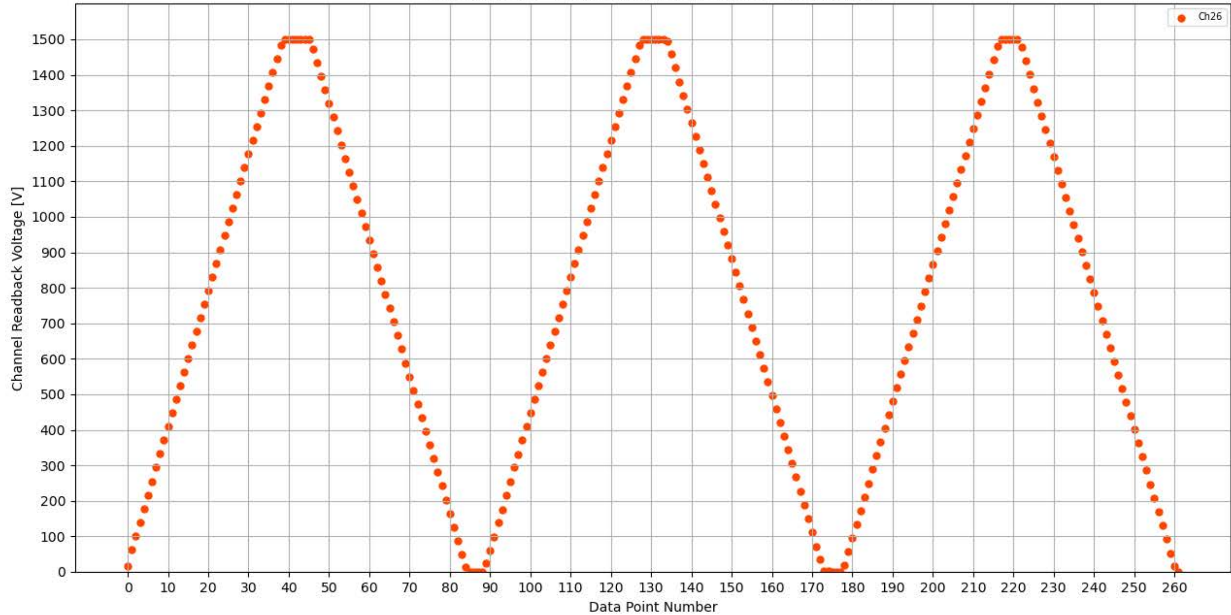
Voltage Ramp Test (Python) Bd #339, Slot #10, Ch #26
