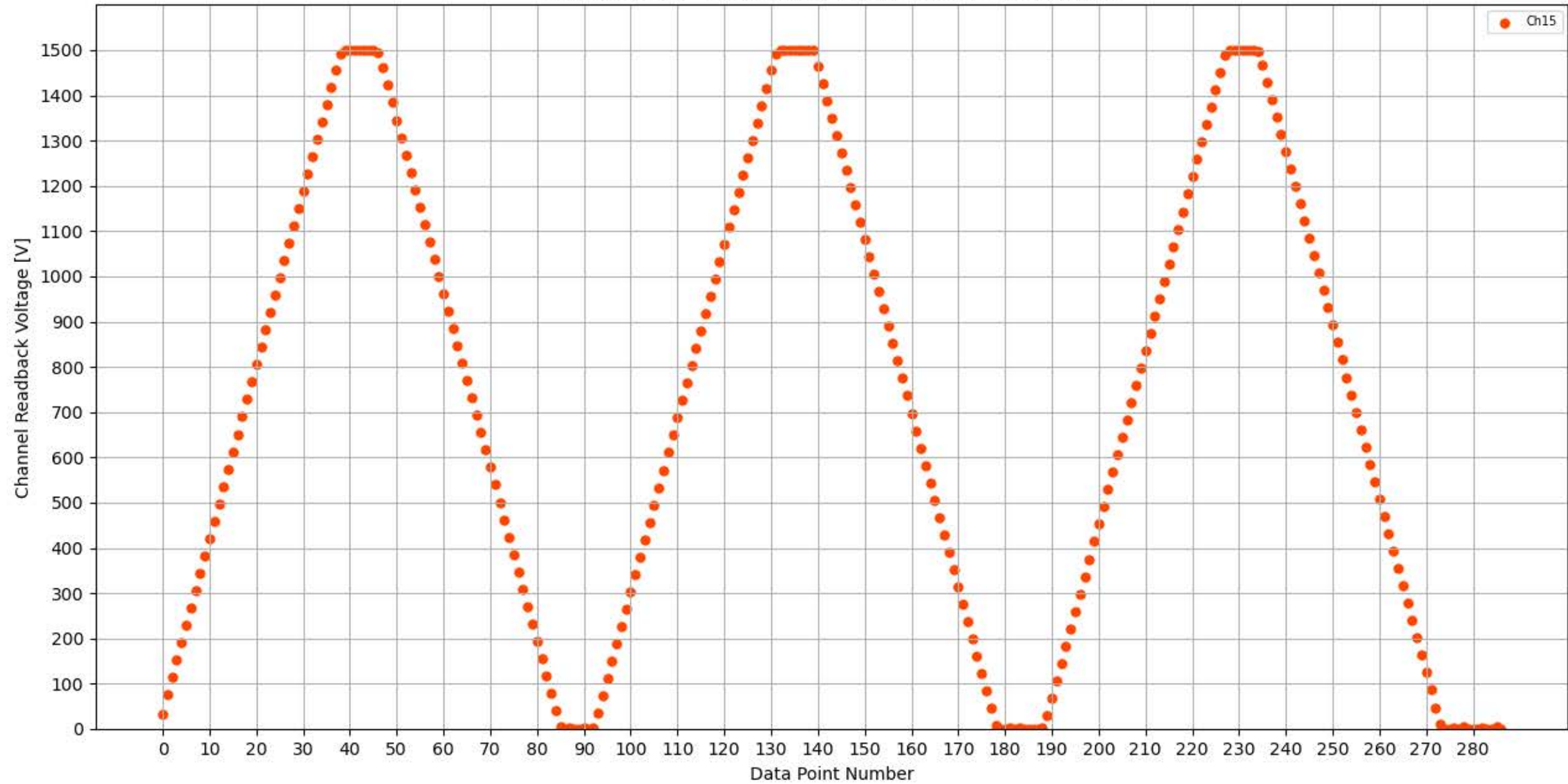
Voltage Ramp Test (Python) Bd #339, Slot #10, Ch #15
