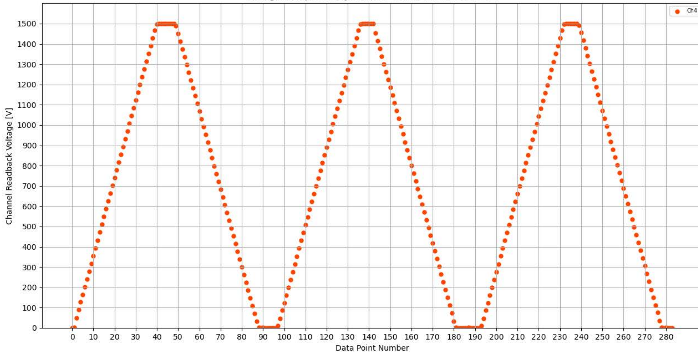
Voltage Ramp Test (Python) Bd #339, Slot #10, Ch #4
