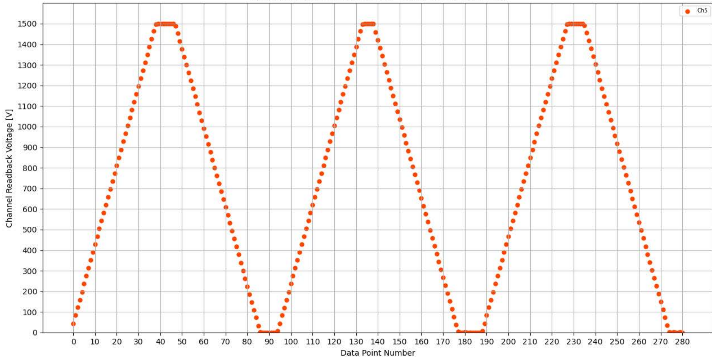
Voltage Ramp Test (Python) Bd #339, Slot #10, Ch #5
