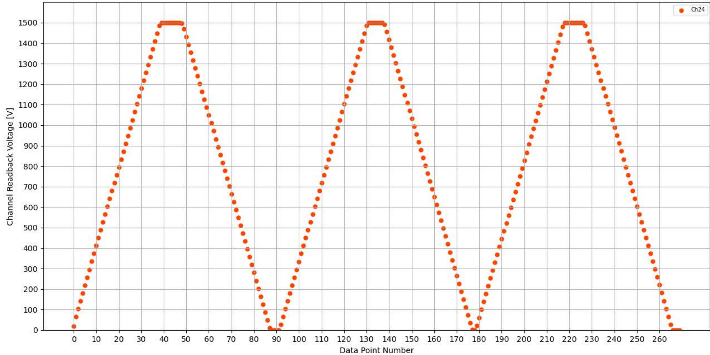
Voltage Ramp Test (Python) Bd #339, Slot #10, Ch #24
