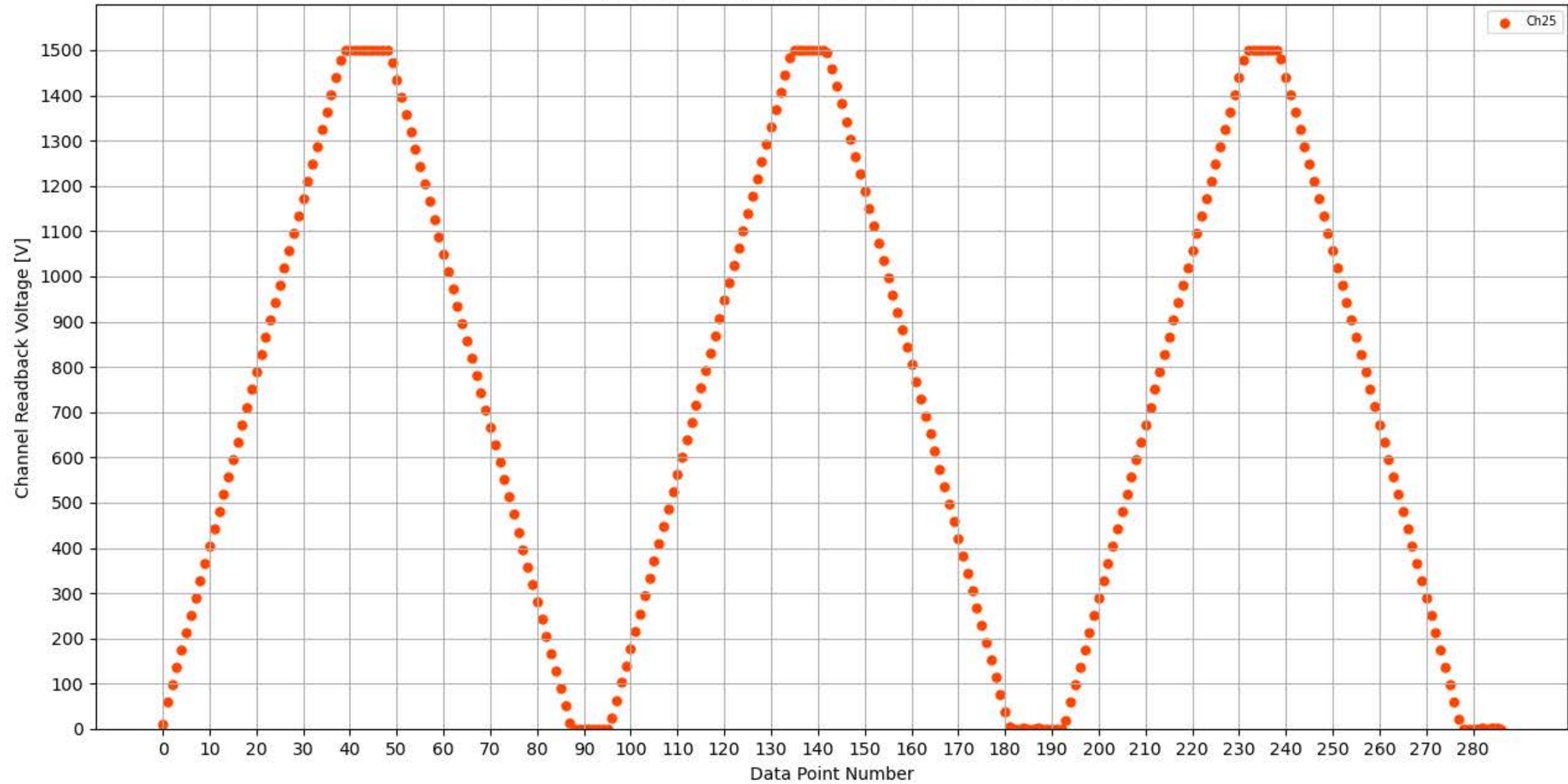
Voltage Ramp Test (Python) Bd #339, Slot #10, Ch #25
