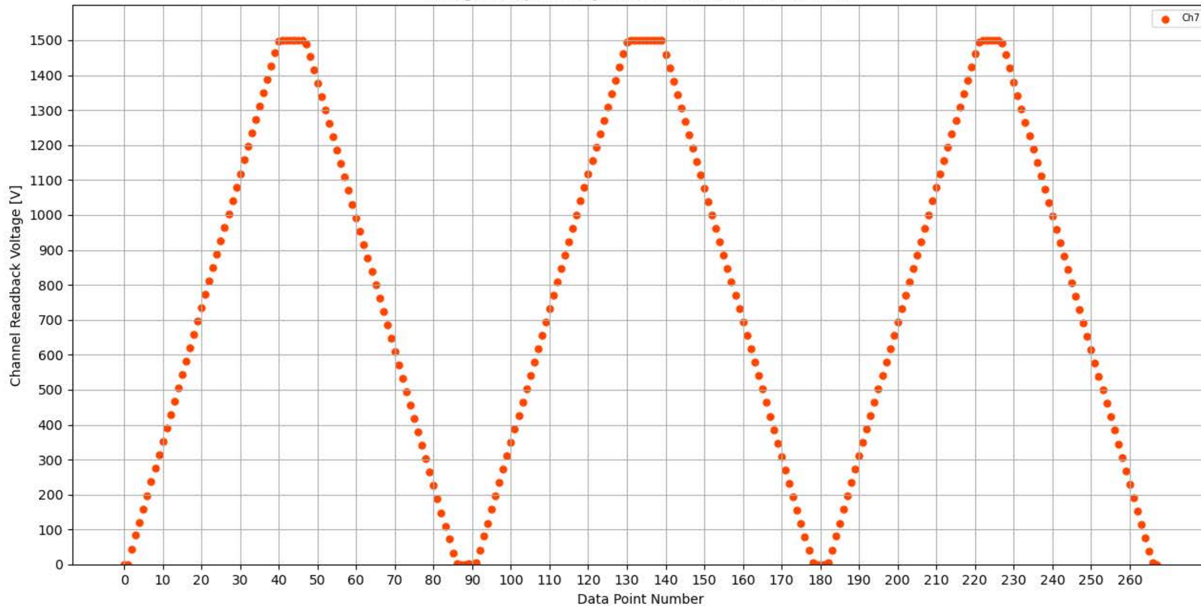
Voltage Ramp Test (Python) Bd #339, Slot #10, Ch #7
