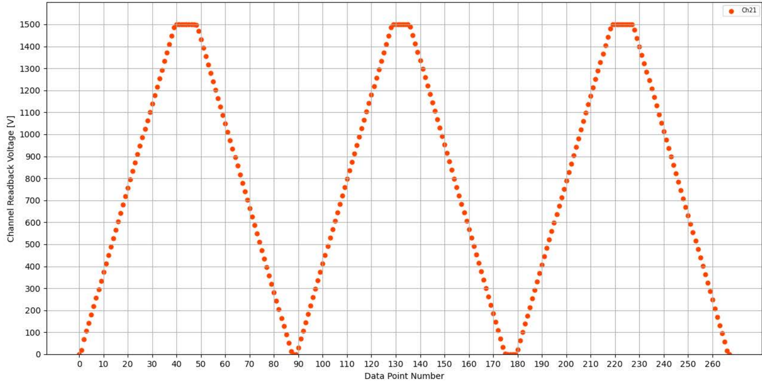
Voltage Ramp Test (Python) Bd #339, Slot #10, Ch #21
