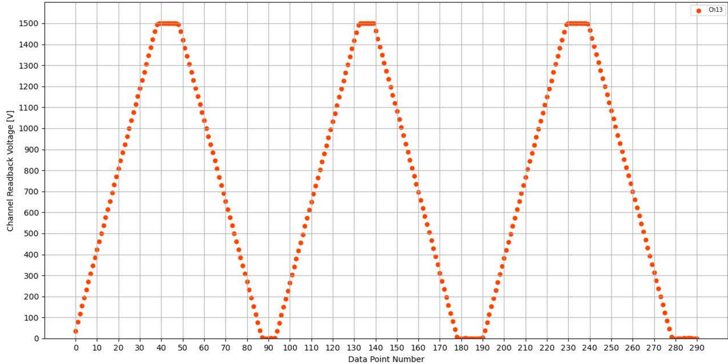
Voltage Ramp Test (Python) Bd #339, Slot #10, Ch #13
