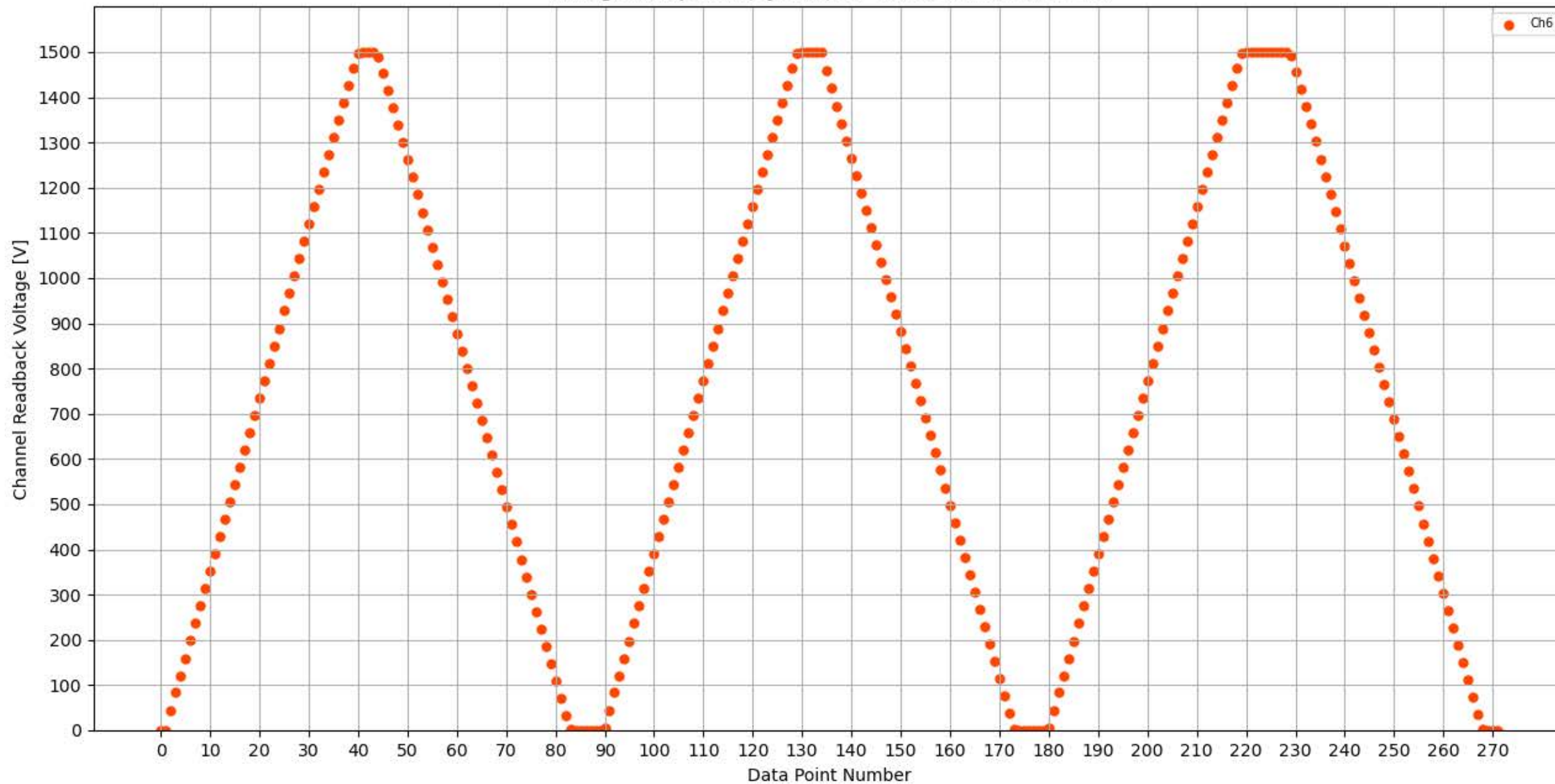
Voltage Ramp Test (Python) Bd #339, Slot #10, Ch #6
