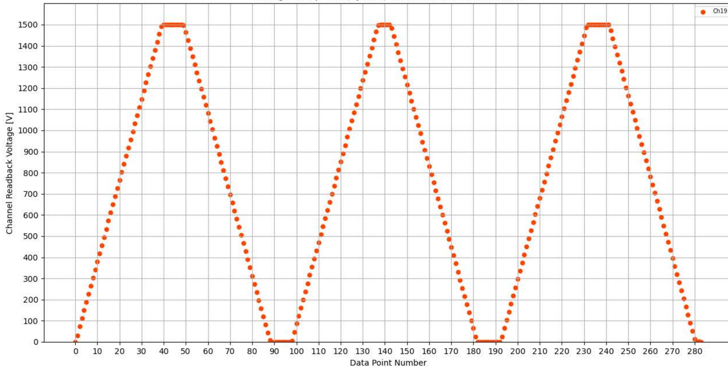
Voltage Ramp Test (Python) Bd #339, Slot #10, Ch #19
