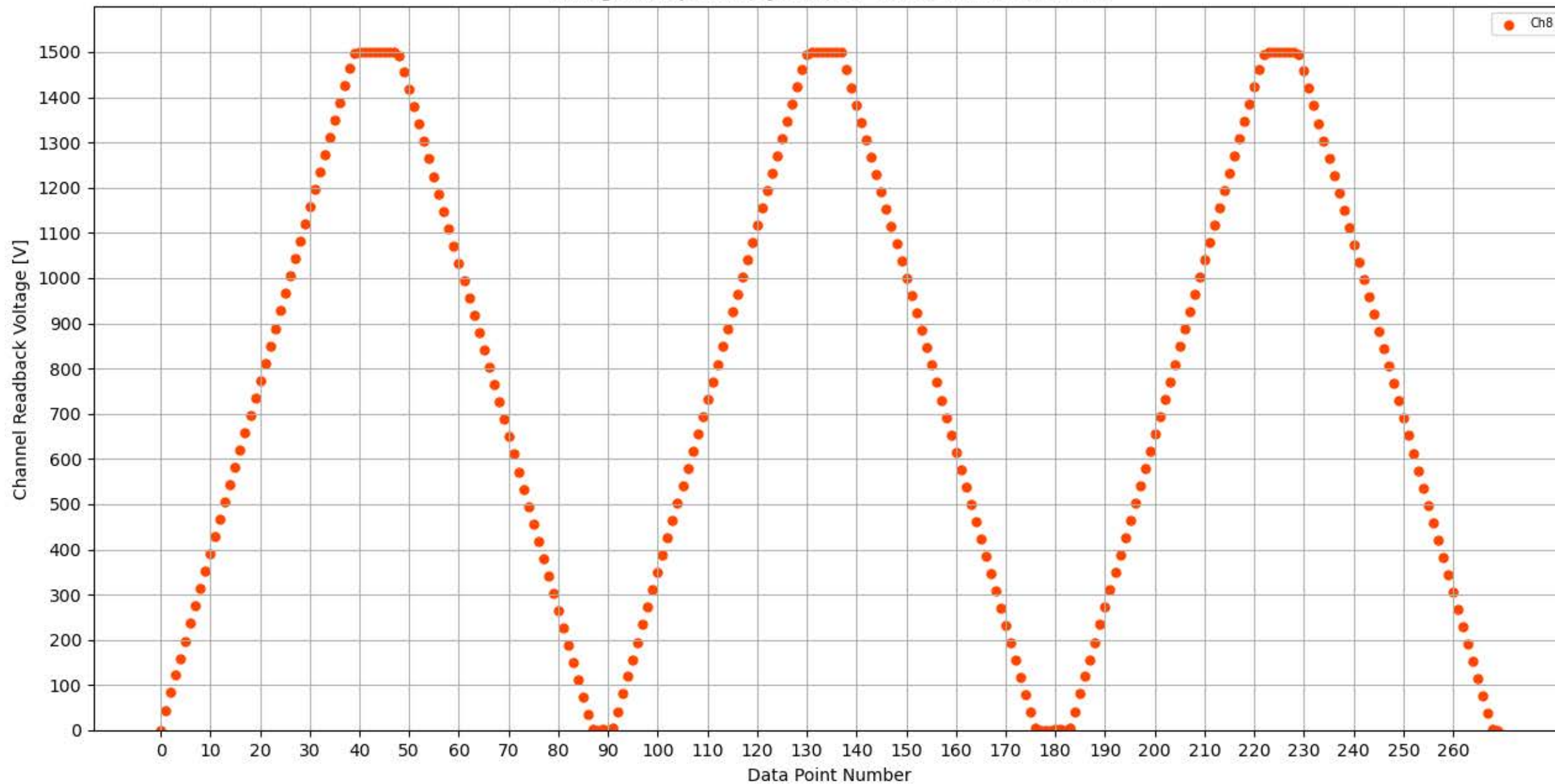
Voltage Ramp Test (Python) Bd #339, Slot #10, Ch #8
