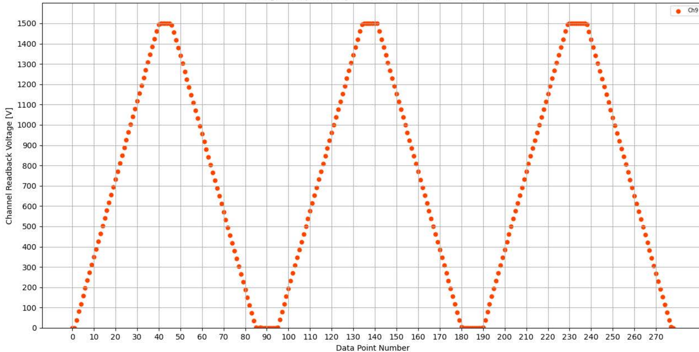
Voltage Ramp Test (Python) Bd #339, Slot #10, Ch #9
