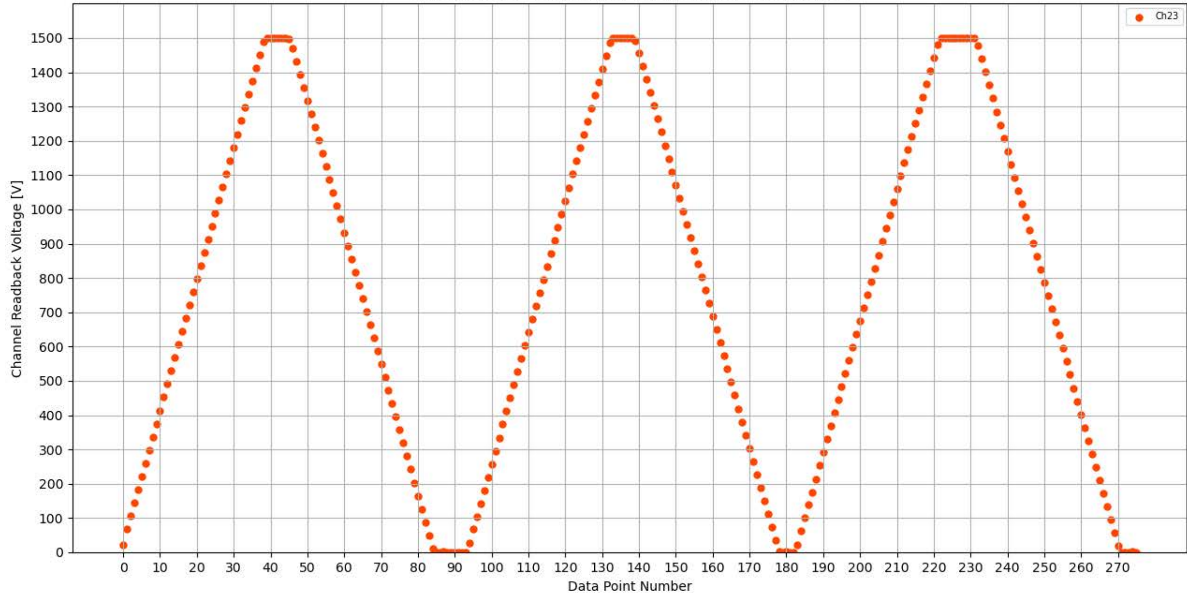
Voltage Ramp Test (Python) Bd #339, Slot #10, Ch #23
