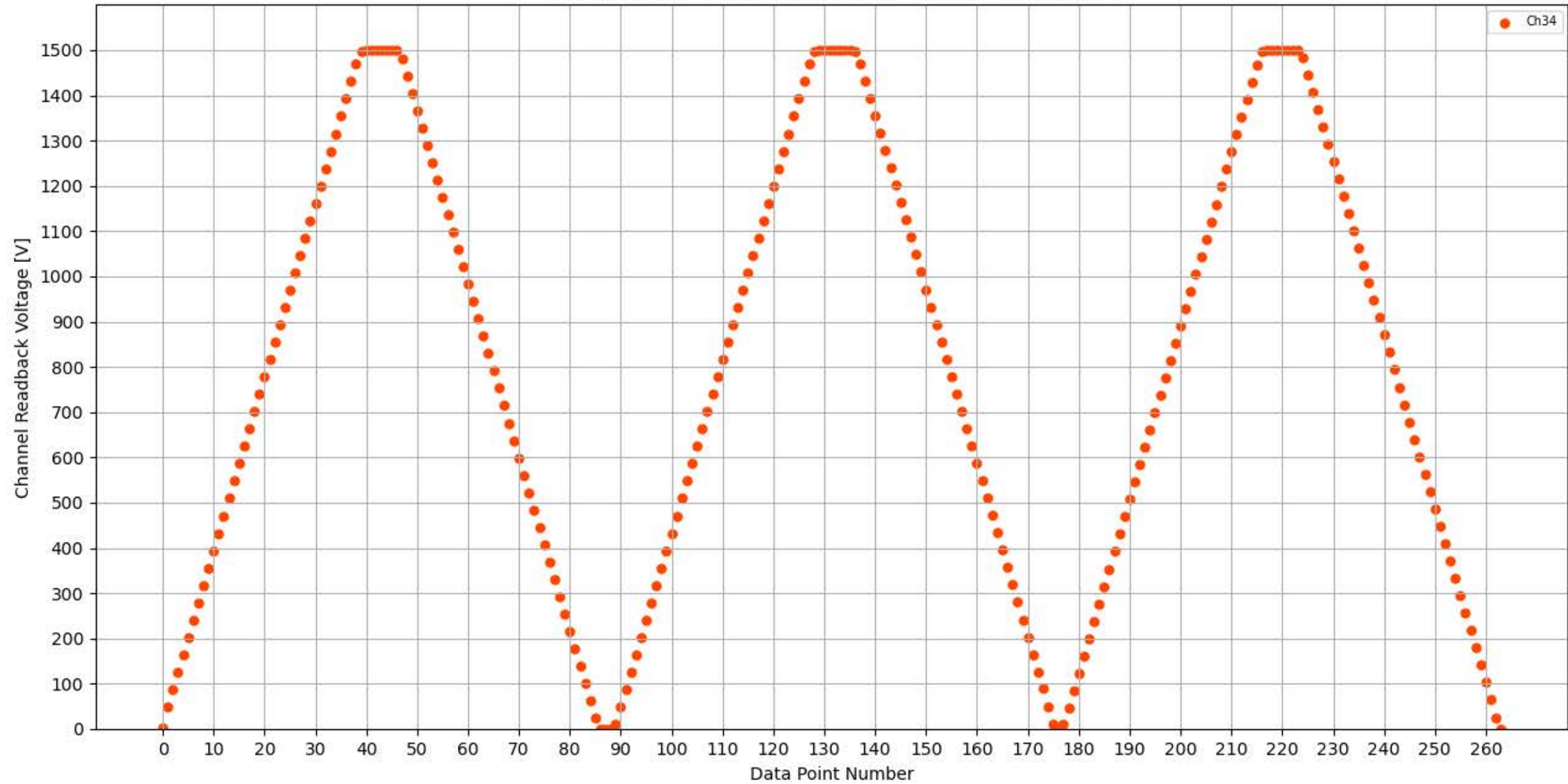
Voltage Ramp Test (Python) Bd #339, Slot #10, Ch #34
