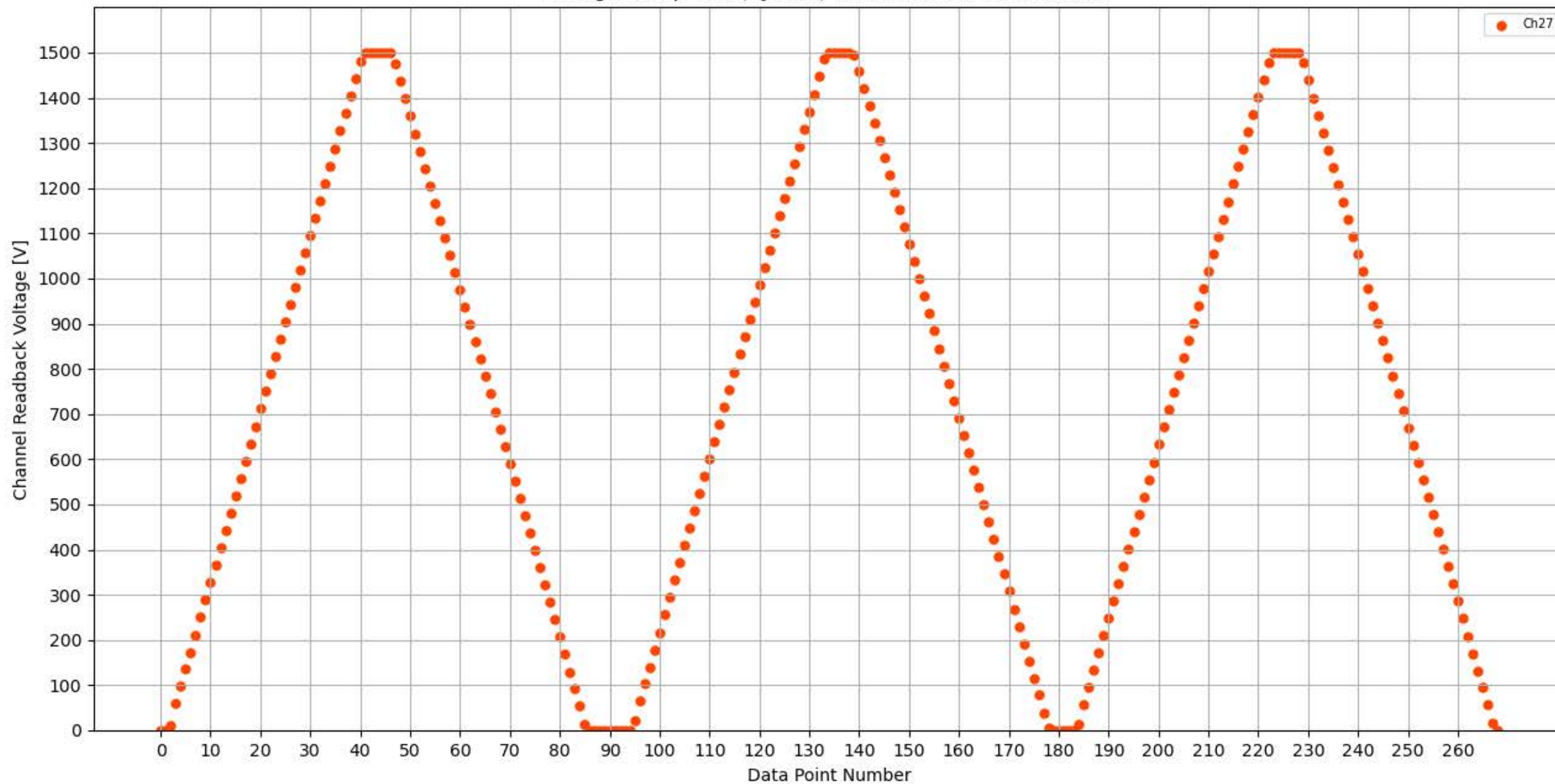
Voltage Ramp Test (Python) Bd #339, Slot #10, Ch #27
