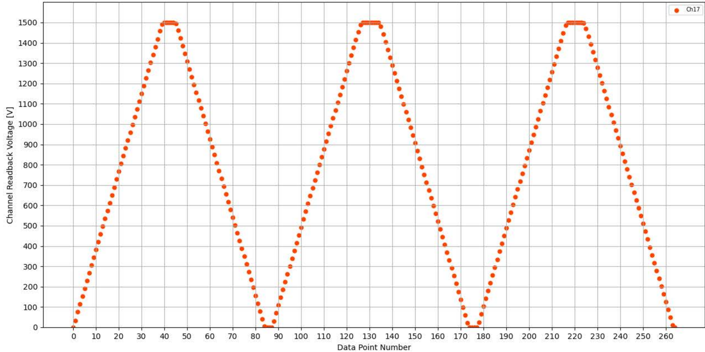
Voltage Ramp Test (Python) Bd #339, Slot #10, Ch #17
