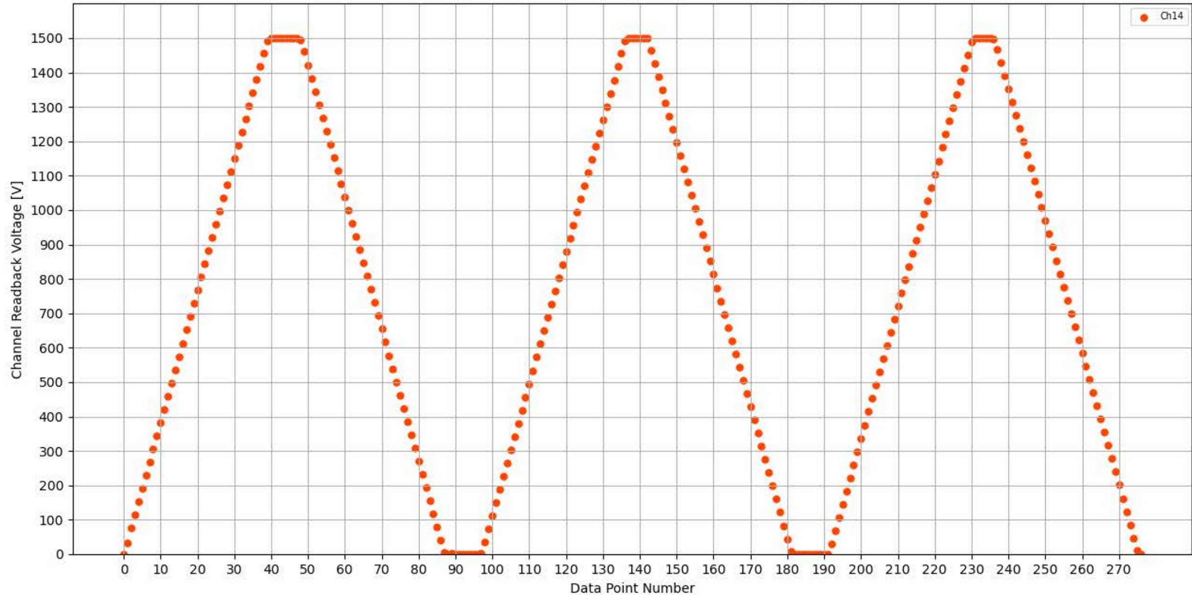
Voltage Ramp Test (Python) Bd #339, Slot #10, Ch #14
